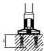
supporting leg screwed to floor with nylon cover sleeve drilling depth min. 35mm
